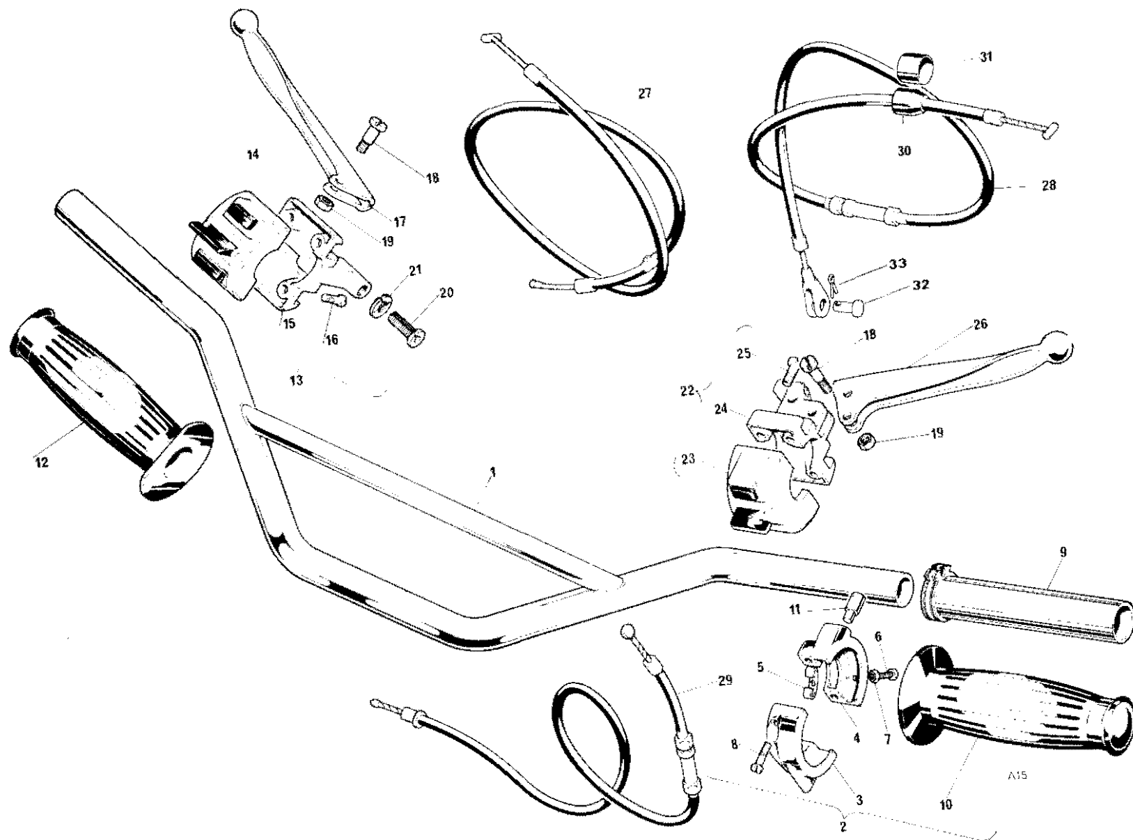
Fig. 15. HANDLEBARS, CONTROL LEVERS AND CABLES
