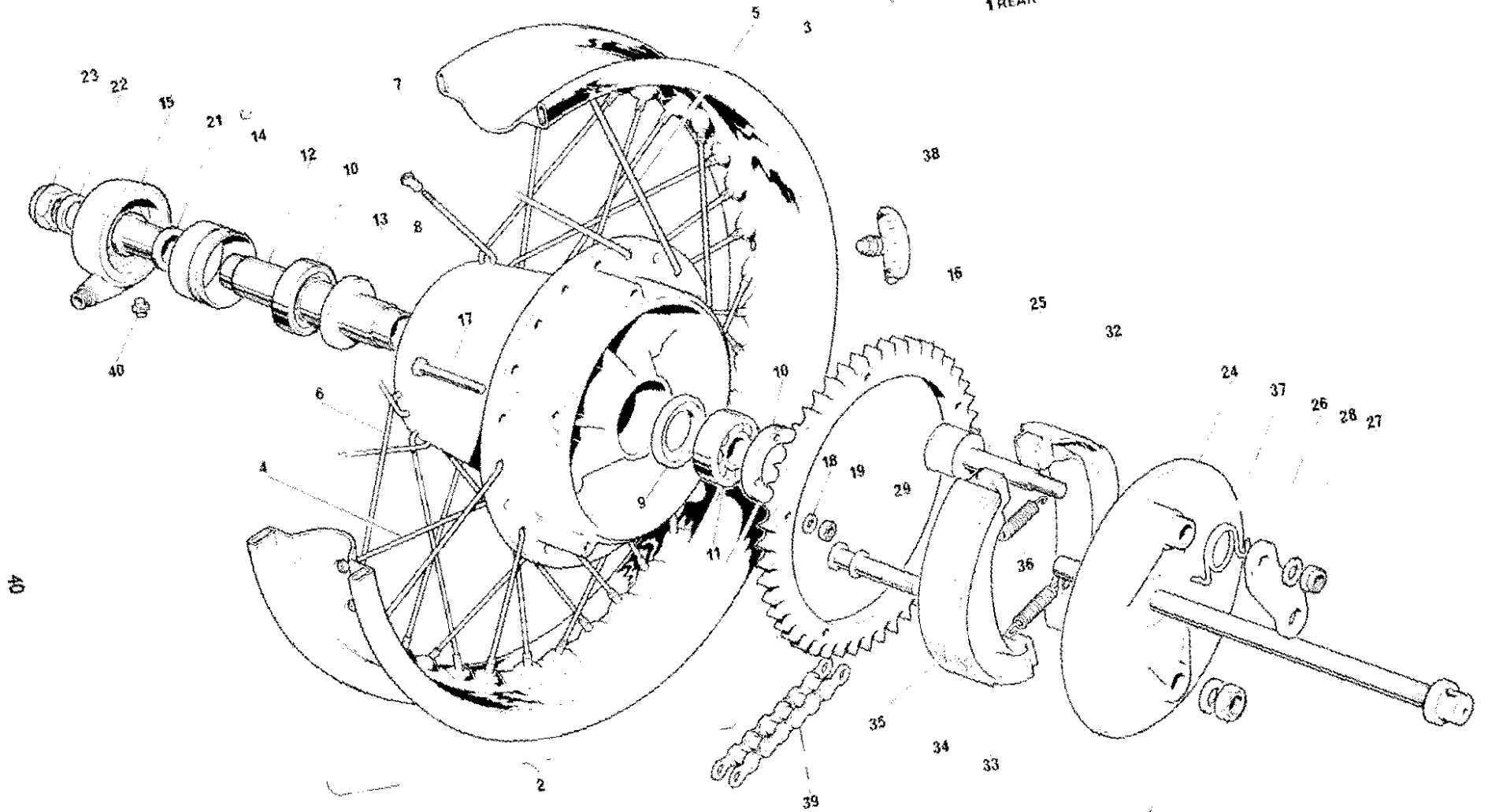
Fig. 12. REAR WHEEL
