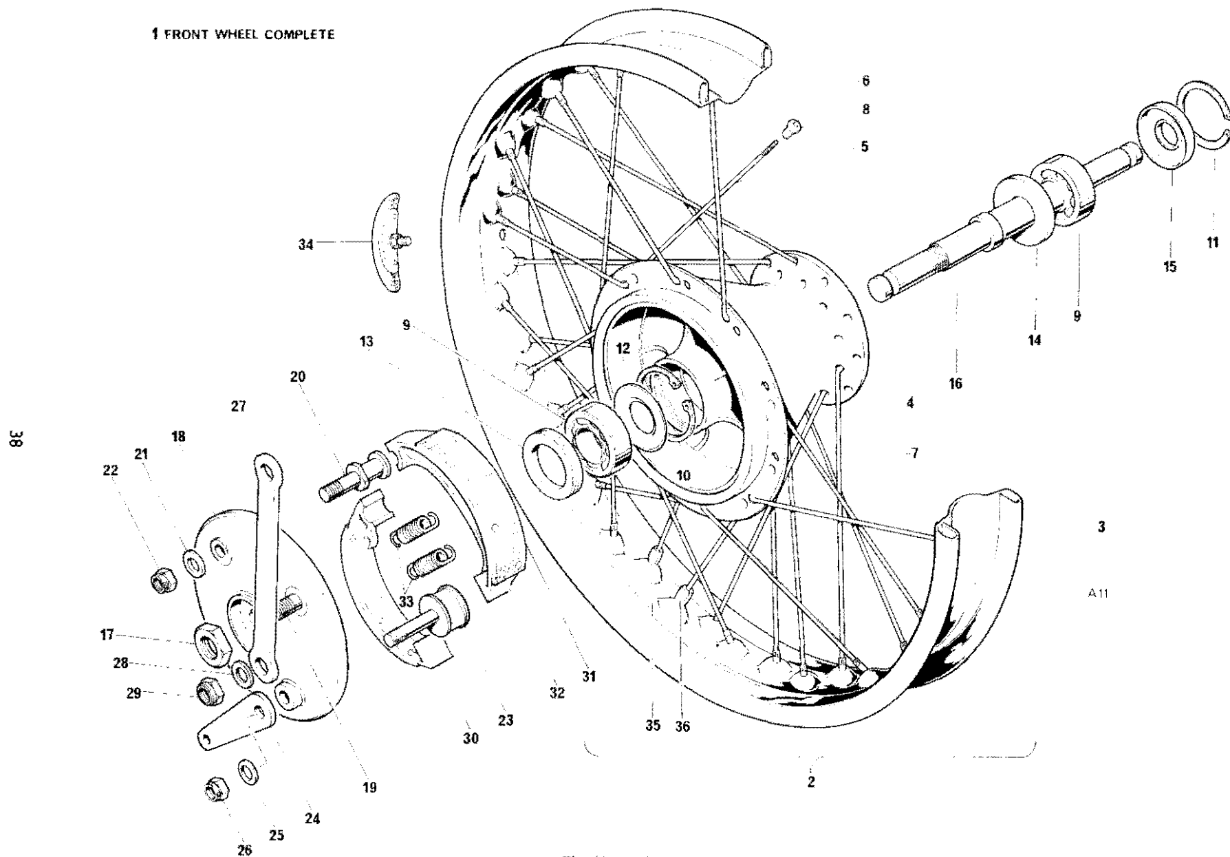
Fig. 11. FRONT WHEEL
