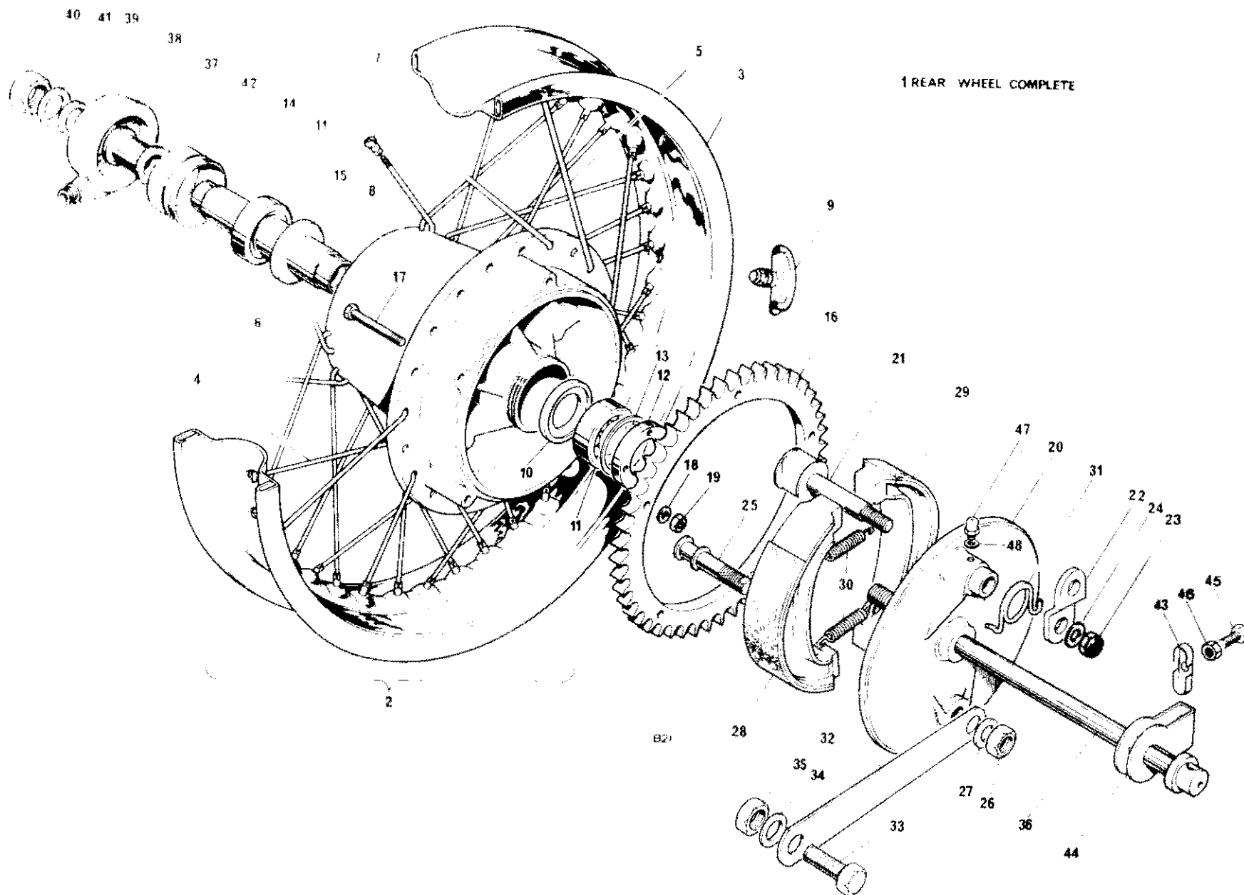
Fig 24. REAR WHEEL
